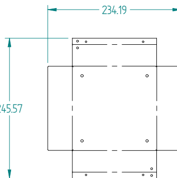
FLAT PATTERN
