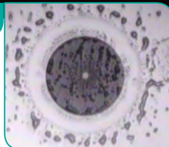
Dirty F-O connector after mating
